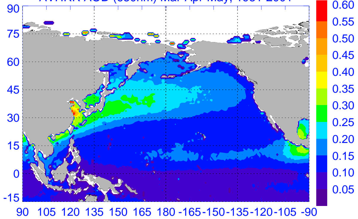
AVHRR AOD (630nm) Mar-Apr-May, 1981-2001
